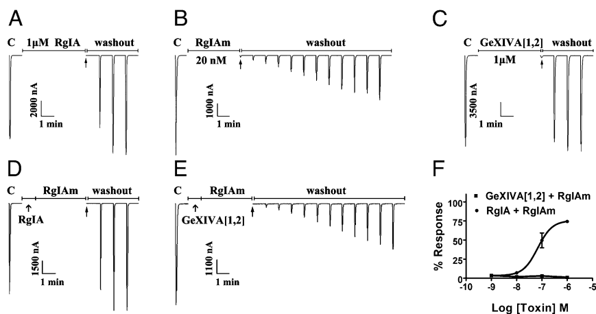
Fig. 3. Binding site comparison of \alpha O-GeXIVA and \alpha -conotoxin RgIA. In each instance, toxin solution was applied to \alpha 9 \alpha 10 nAChRs expressed in Xenopus oocytes, followed by toxin washout. The response to 1-s pulses to ACh were measured as described in Materials and Methods . (A) One micromolar \alpha -conotoxin RgIA for 5 min. Note the rapid recovery following toxin washout. (B) Twenty nanomolar \alpha -conotoxin RgIA for 4 min. Note the slow recovery. (C) One micromolar \alpha O-conotoxin GeXIVA[1,2] for 5 min. Note the rapid recovery. (D) One micromolar \alpha -conotoxin RgIA for 1 min, followed by 20 nM \alpha -conotoxin RgIA for 4 min. Note that preblockade of \alpha 9 \alpha 10 nAChR with \alpha -conotoxin RgIA prevented the slowly reversible block associated with \alpha -conotoxin RgIA, consistent with competitive binding to the same or overlapping site. (E) One micromolar \alpha O-GeXIVA[1,2] for 1 min, followed by 20 nM \alpha -conotoxin RgIA for 4 min. Note that preblockade of \alpha 9 \alpha 10 nAChR with \alpha O-GeXIVA[1,2] did not prevent the very slowly reversible block associated with \alpha -conotoxin RgIA, consistent with occupancy of distinct binding sites. (F) Oocytes expressing \alpha 9 \alpha 10 nAChRs were preincubated with varying concentrations of RgIA for 5 min. This step was followed by coincubation with RgIA + 20 nM RgIA for a further 5 min. Both toxins were then washed out, and the response was measured following 2 min of washout. Note that an increasing concentration of RgIA led to a greater percent response (faster recovery) to ACh. Oocytes expressing \alpha 9 \alpha 10 nAChRs were preincubated with varying concentrations of GeXIVA[1,2] for 5 min. This step was followed by coincubation with GeXIVA[1,2] + 20 nM RgIA for a further 5 min. Both toxins were then washed out, and the response was measured following 2 min of washout. Note that an increasing concentration of GeXIVA[1,2] had no effect on percent response to ACh ( n = 5-6 oocytes).
